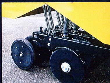
Rugged double disc opener with "T" handle adjustable presswheel
